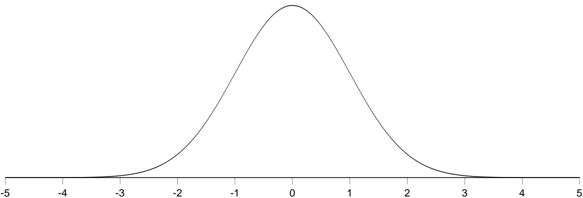
Normal Distribution
